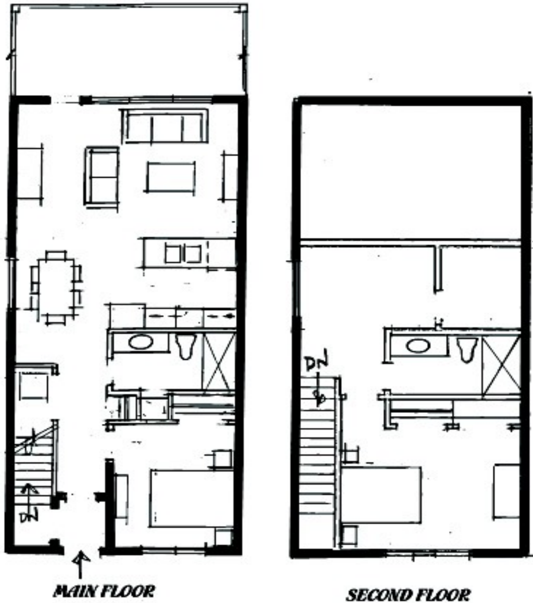
FLOOR PLAN - SECOND FLOOR LOFT UNIT - 1262 S.F.
